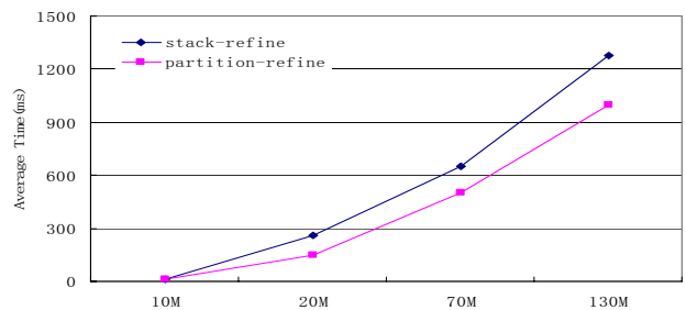
Fig. 7 Processing time with increasing document size
