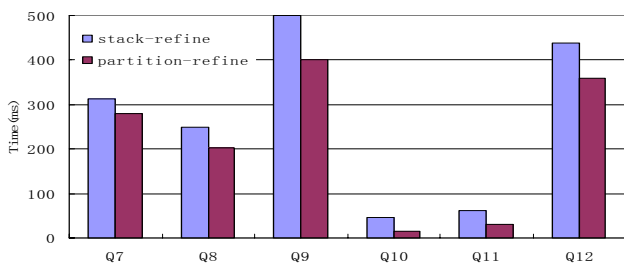
Fig. 5 Processing time on DBLP
