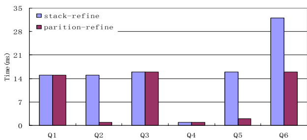
Fig. 4 Processing time on SIGMOD Record
