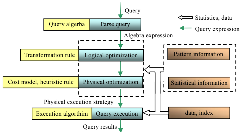
Fig.1 Query Processing
