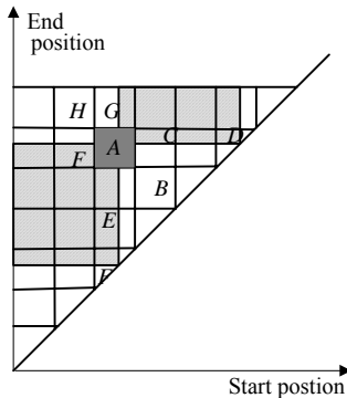
Fig.6 Two-Dimension histogram
