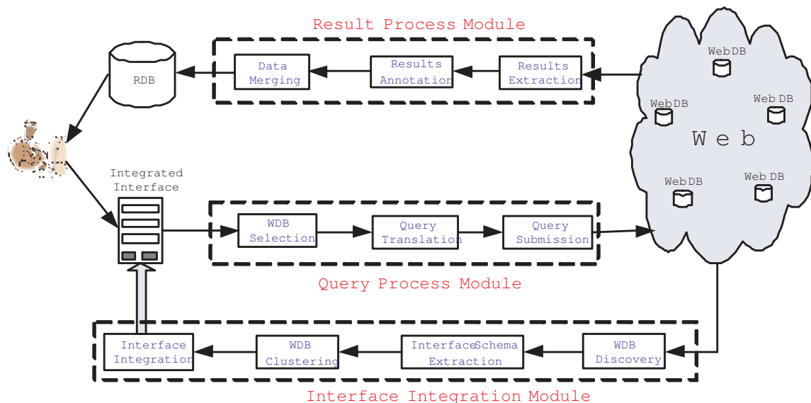
Figure 2: A comprehensive solution for Web database integration
