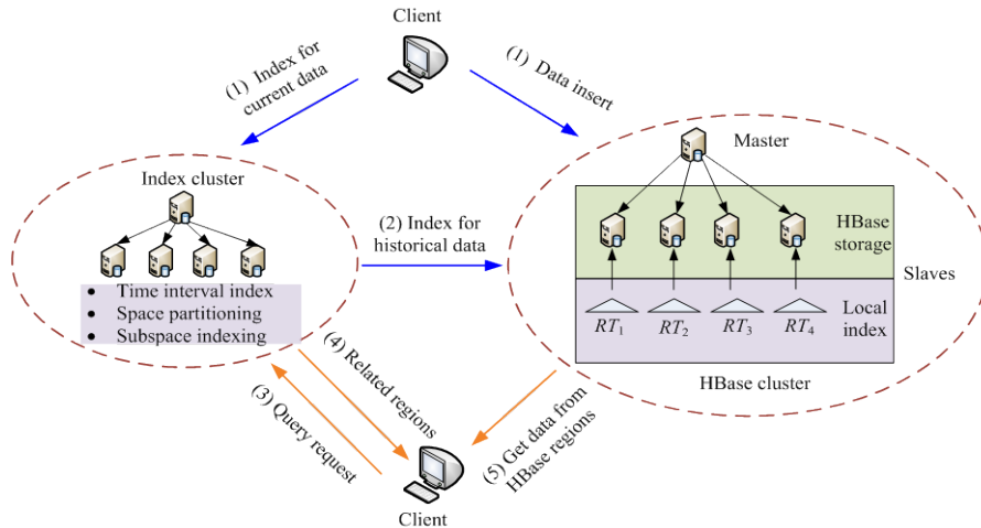
Fig.15 System architecture
