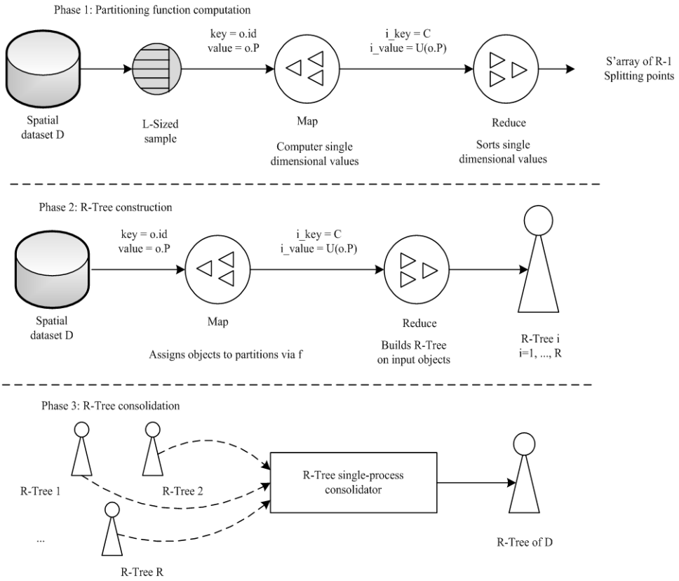
Fig.12 Index procedure
