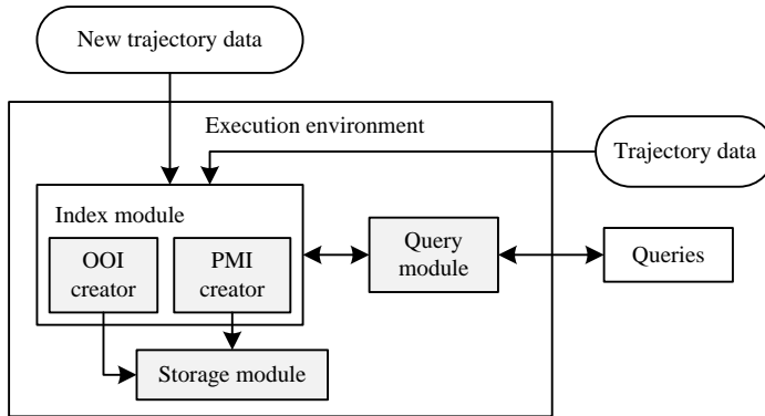
Fig.9 Processing framework of trajectory data
