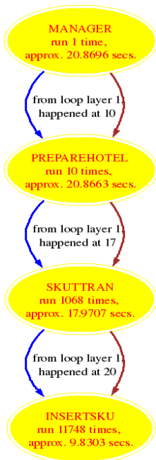
Figure 25. Output of AppSleuth for the original application code as well as the trace.
