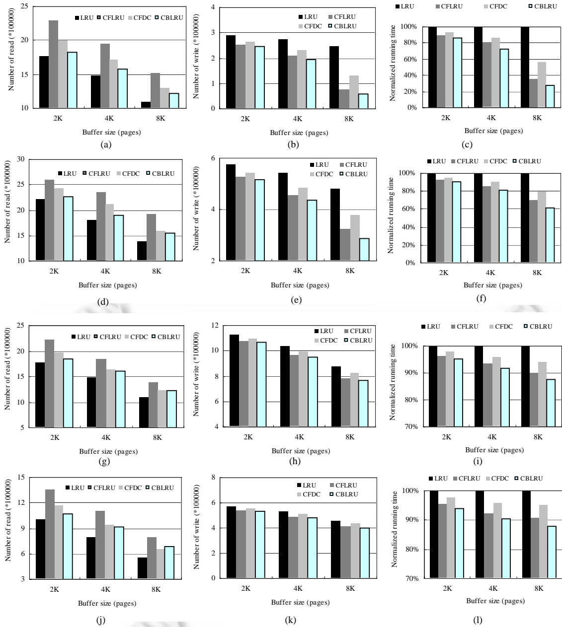
Fig.7 Comparison of read, write and running time for different methods when executing T1 to T4 on FD1
