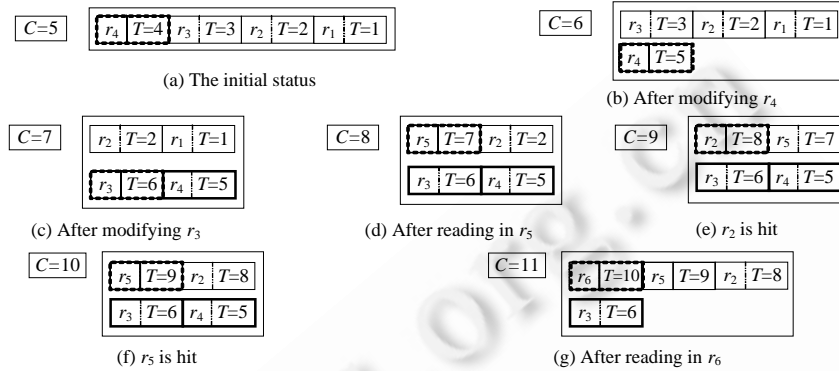
Fig.6 Illustration of the optimized CBLRU for sequence r_1, r_2, r_3, r_4, r_4, r_3, r_5, r_2, r_5, r_6
