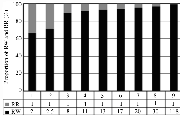
Fig.1 Normalized proportion of time consumed by random write (RW) and random read (RR) operations for NAND flash disks
