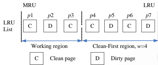
Fig.2 CFLRU replacement policy 图 2 CFLRU 置换策略示意图
