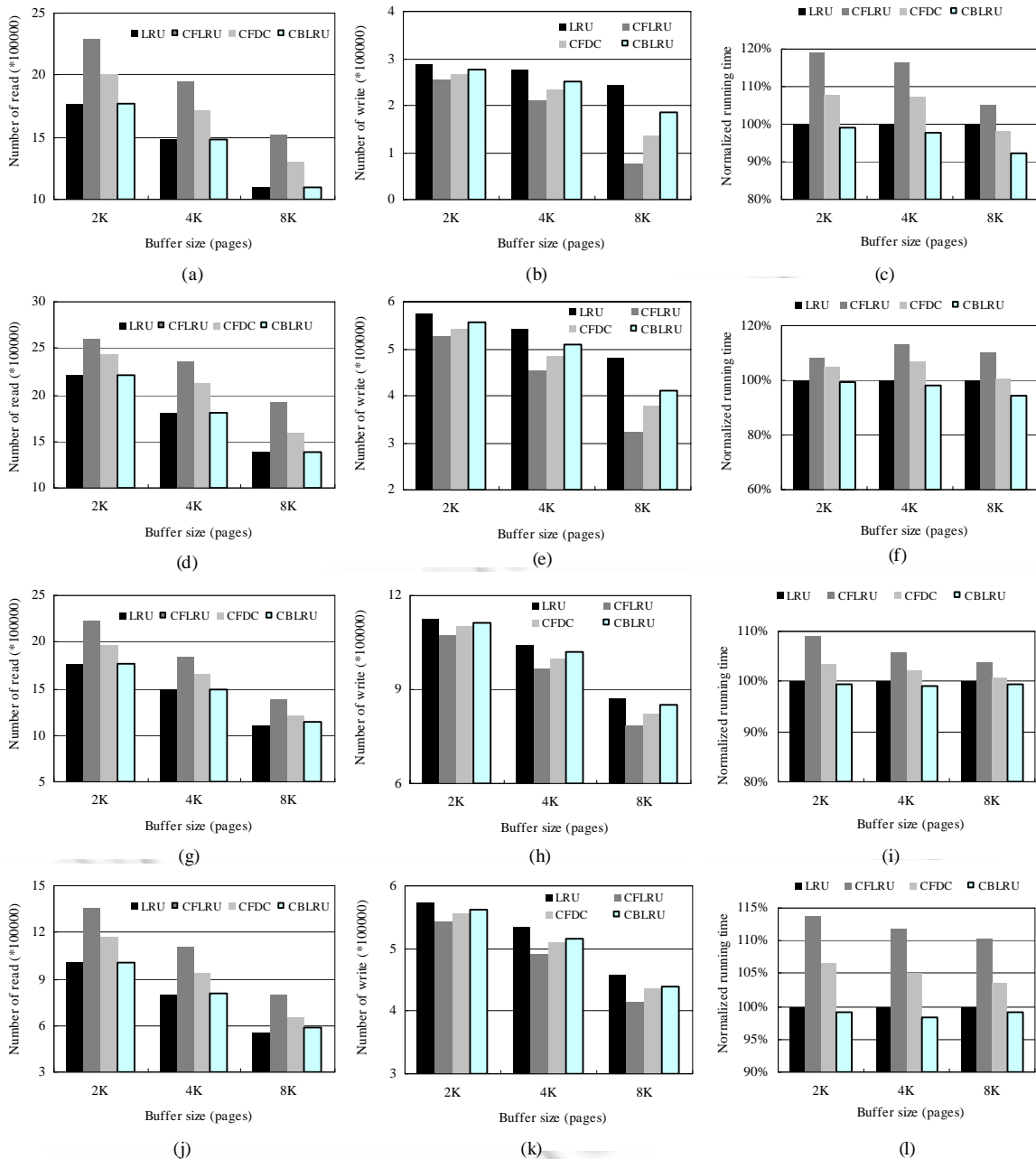
Fig.8 Comparison of read, write and running time for different methods when executing T_1 to T_4 on FD2
