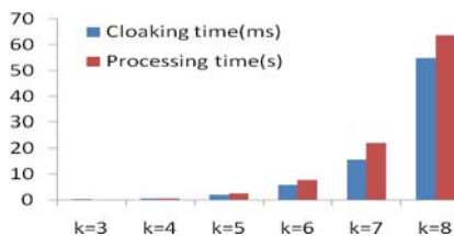
Fig.9 Cloaking time and processing time
