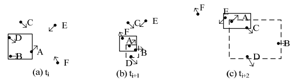
Fig.2 Privacy preserving for continuous query. (a) t_i ; (b) t_{i+1} ; (c) t_{i+2} 图 2 连续查询隐私保护. (a) t_i ; (b) t_{i+1} ; (c) t_{i+2}
