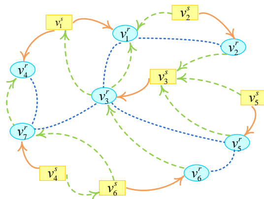
Fig.3 S-R credibility network
